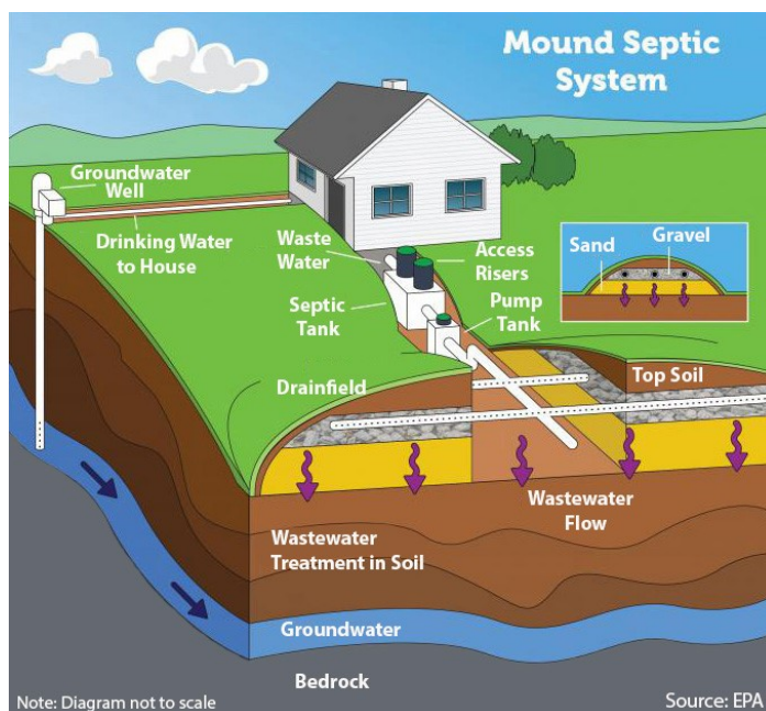
Figure 4. Diagram of a mound soil dispersal system. A mound is used in areas with poorer quality soils or high-water tables to provide needed wastewater to soil contact and treatment.
