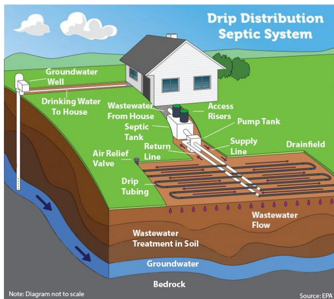
Figure 5. Diagram of a drip dispersal system. Wastewater is pumped from pumping chamber to drip tubes typically placed shallow in the soil.
