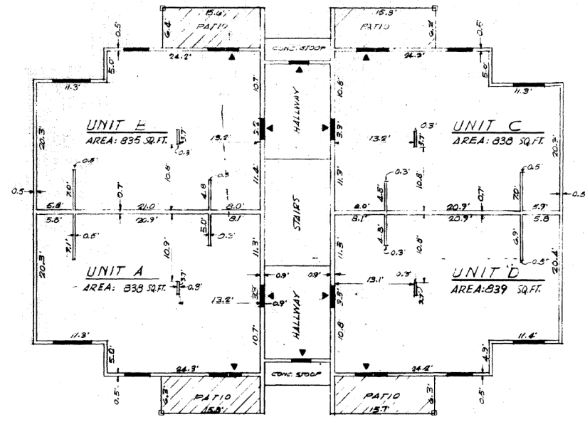
FIRST FLOOR FLOOR ELEV. 478.00 CLG. ELEV. 484.10 PATIO ELEV. 477.0
