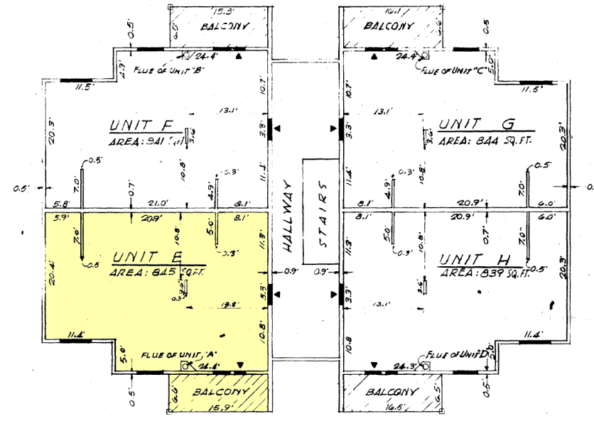
SECOND FLOOR FLOOR ELEV. 487.30 CLG. ELEV. 495.50 BALCONY ELEV. 487.1
