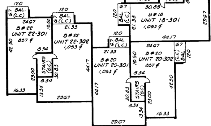
3RD FLOOR
