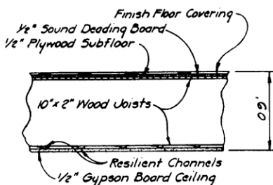
FLOOR DETAIL
